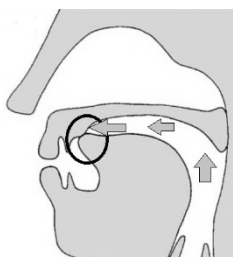
Figure 2-8 /t/ /d/
