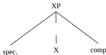
Figure 6-15 XP Rule
