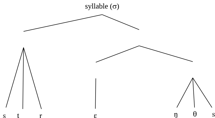
Figure 3-4 Syllable structure
