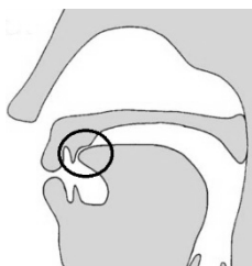
Figure 2-10 /s/ /z/
